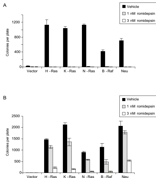
Figure 4 Romidepsin inhibits anchorage-independent growth of transformed NIH 3T3 and RIE-1 cells. NIH 3T3 cells (A) and RIE-1 cells (B) stably expressing the indicated proteins were evaluated for colony formation in soft agar in complete growth medium supplemented with the indicated concentrations of romidepsin. Following 23 d (NIH 3T3) or 15 d (RIE-1), viable colonies were stained in MTT and plates were scanned. The number of colonies was quantified from the scanned images using ImageJ software. Data shown are the average ± SD of triplicate plates and are representative of two independent experiments.
